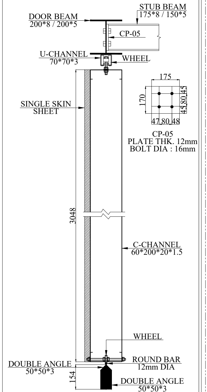
DOUBLE SLIDING DOOR SECTION DETAILS
