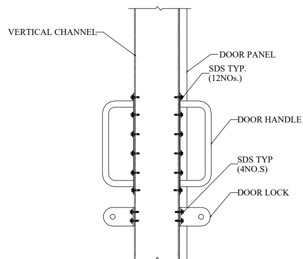
DOOR LOCK AND HANDLE DETAIL
